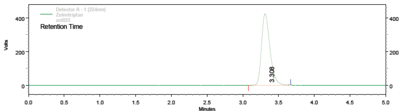
Figure 3: Representative chromatogram of Zolmitriptan (20 µg/ml) Formulation (Zomig tablets, 5 mg).
