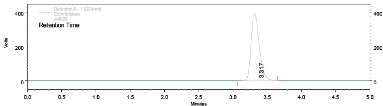
Figure 4: Representative chromatogram of Zolmitriptan (20 µg/ml) Formulation (Zomig ZMT tablets, 2.5 mg)
