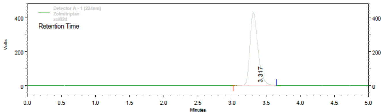
Figure 2: Representative chromatogram of Zolmitriptan (20 \mu\text{g/ml} )
