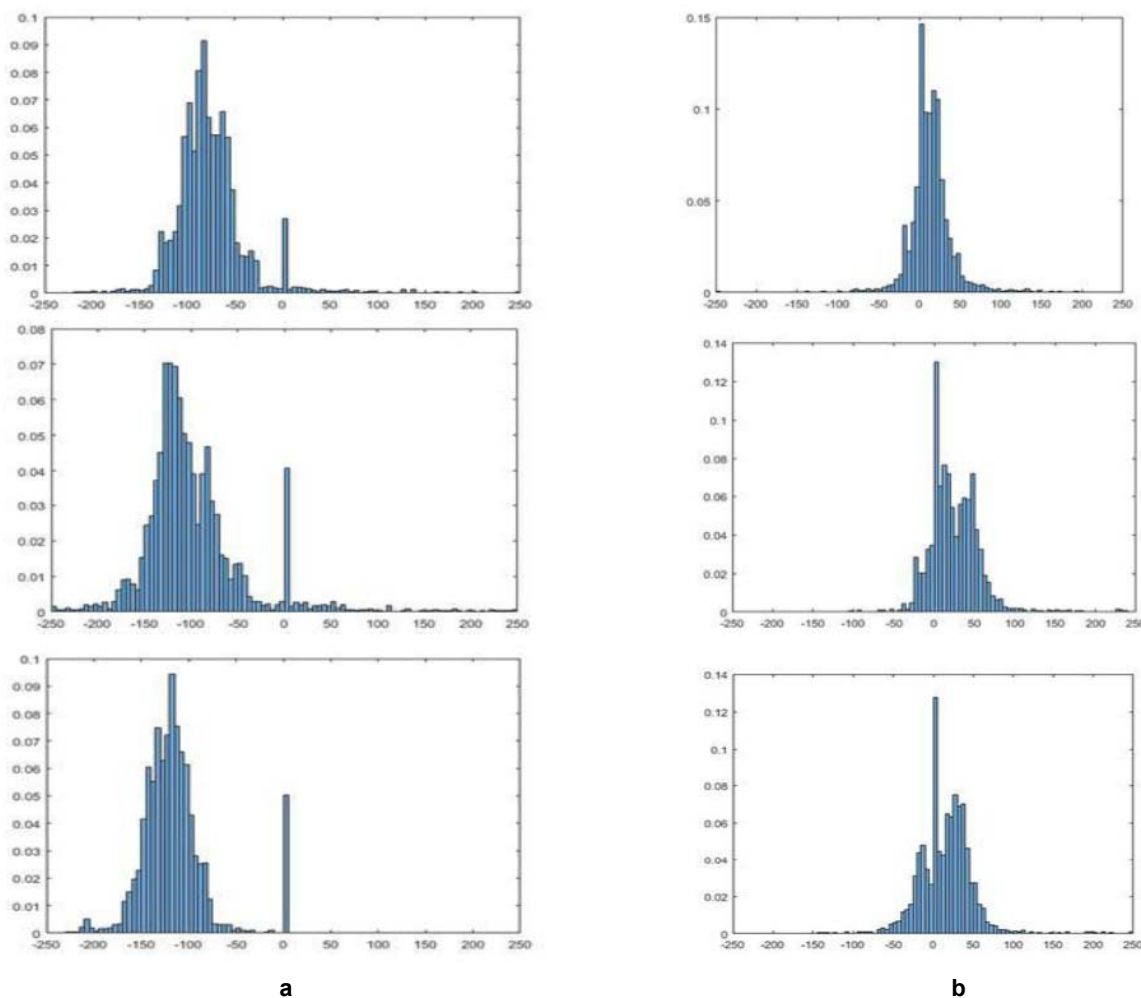
Figure 6: Histograms of two students (vertical rows).
