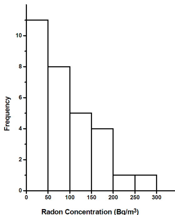
Graph 3: Indoor radon concentrations in dwellings.
